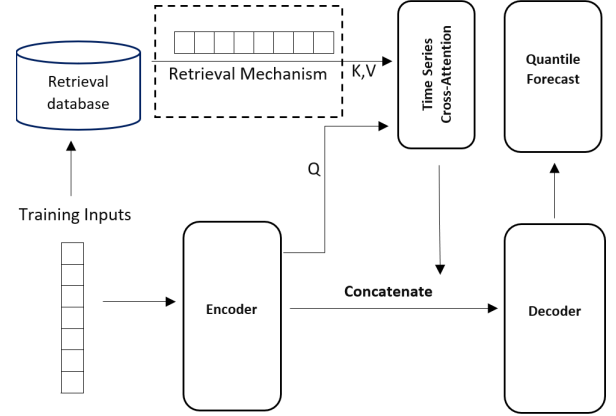
Figure 1: An overview of the MQ-ReTCNN architecture; adapted from [4].
