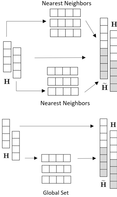
Figure 2: The top diagram depicts nearest neighbor retrieval, the bottom diagram depicts retrieval using a shared global set. The output of the retrieval step is concatenated to the input embedding vector.
